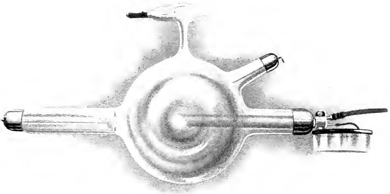
FIG. 30.—Desneur tube with atomiser for cooling the anti-cathode. (Siemens.) This tube is specially exhausted for deep therapeutic work.
